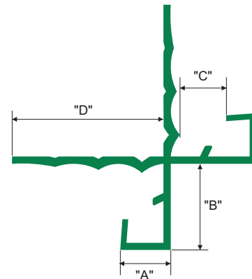
XtremeTrim® Reveal Outside Corner US Patent #9,200,455
