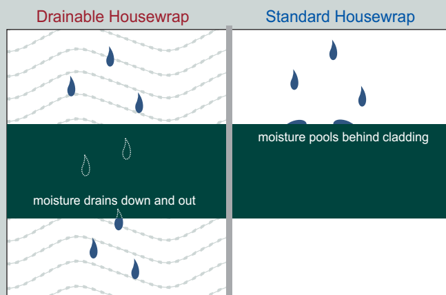
The difference between water-resistive barriers like housewrap and building paper (shown at right) and drainable housewrap (left) is the additional gap created by spacers, which allows moisture to drain from wall assemblies at a faster rate. In addition, the drainage channels form an unobstructed path behind cladding, avoiding the possibility of "ponding" along siding edges with traditional barriers.
